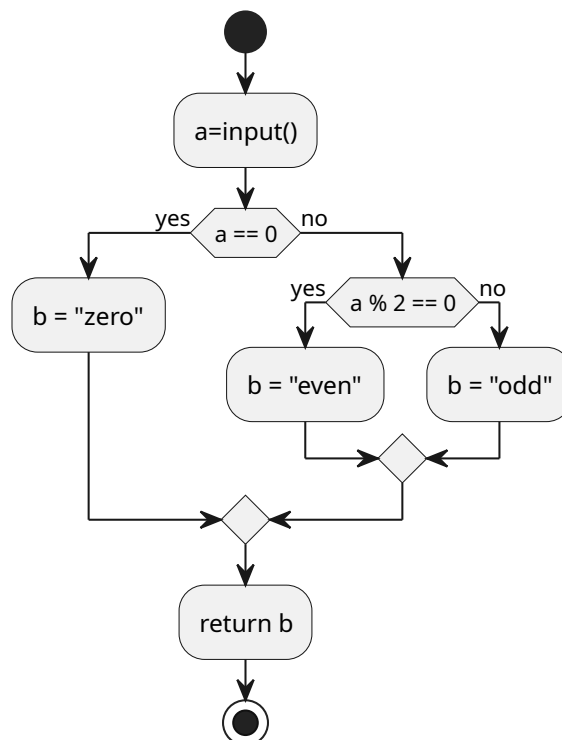
Figure 141: UML of the program which we'll calculate the cyclomatic complexity of
